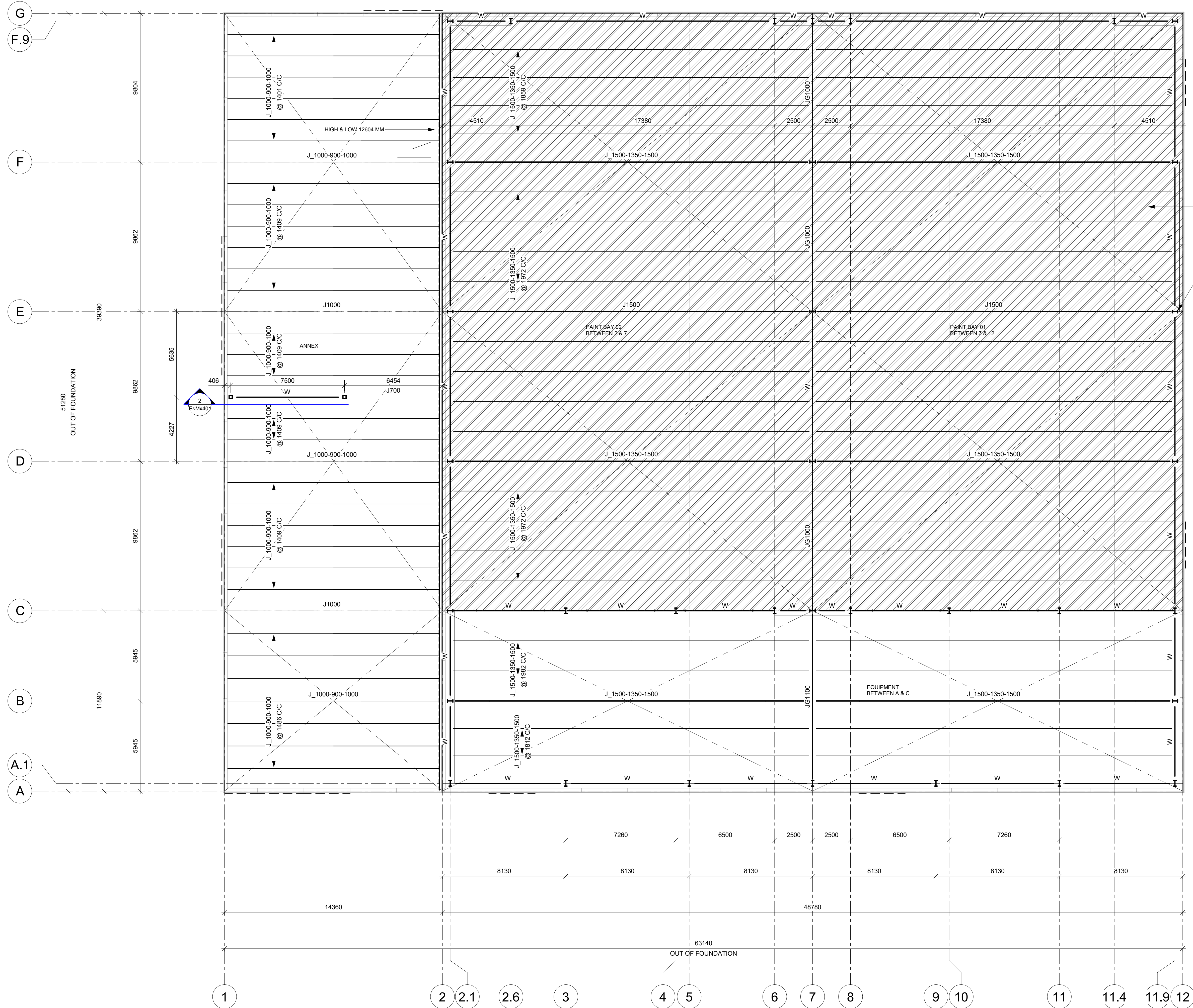
ROOF PLAN 1:125
